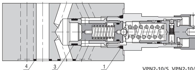
VPN2-10/S, VPN2-10/M
