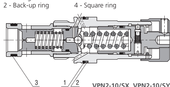
VPN2-10/SX, VPN2-10/SY
