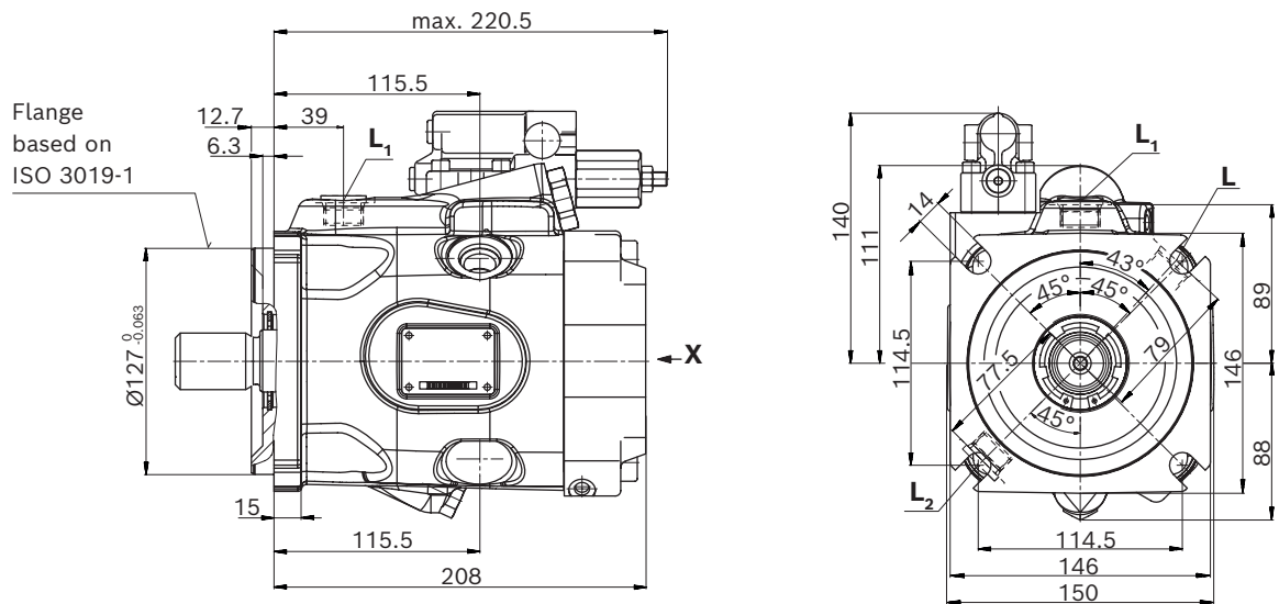
View X 1)
