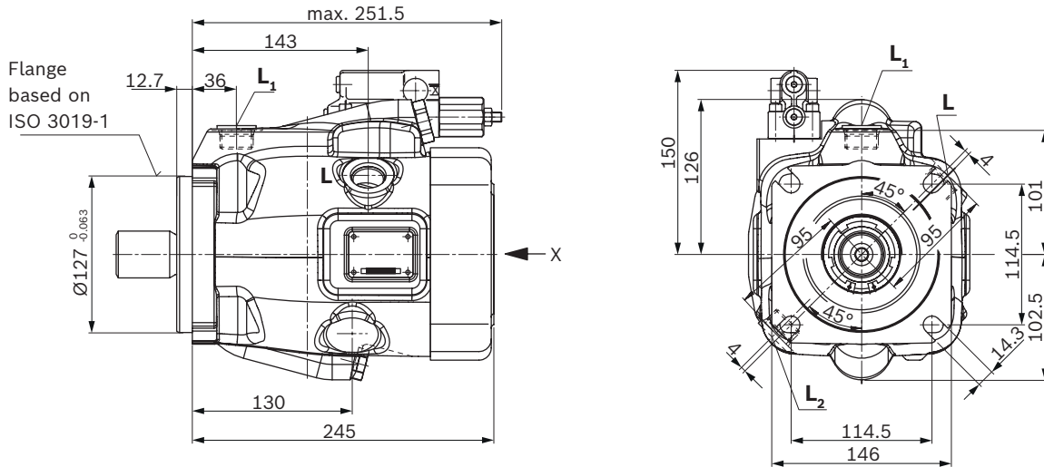
View X 1)
