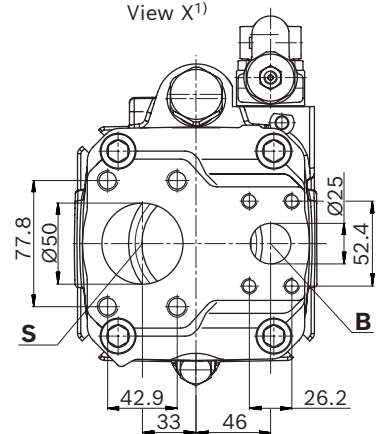
View X 1)
