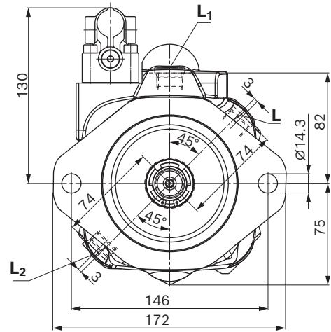
View X 1)
