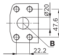
Detail Z
