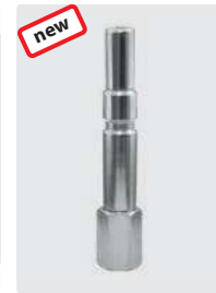
Plug KW : 1/4" F with thread SW17. Stainless steel
